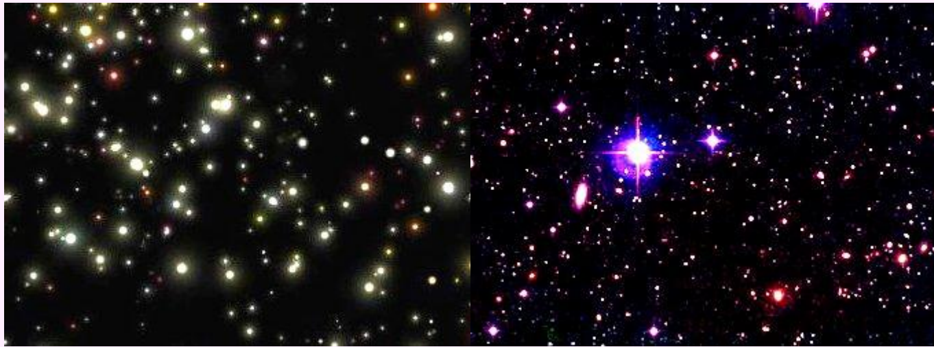
(A - stars) (B - galaxies)
