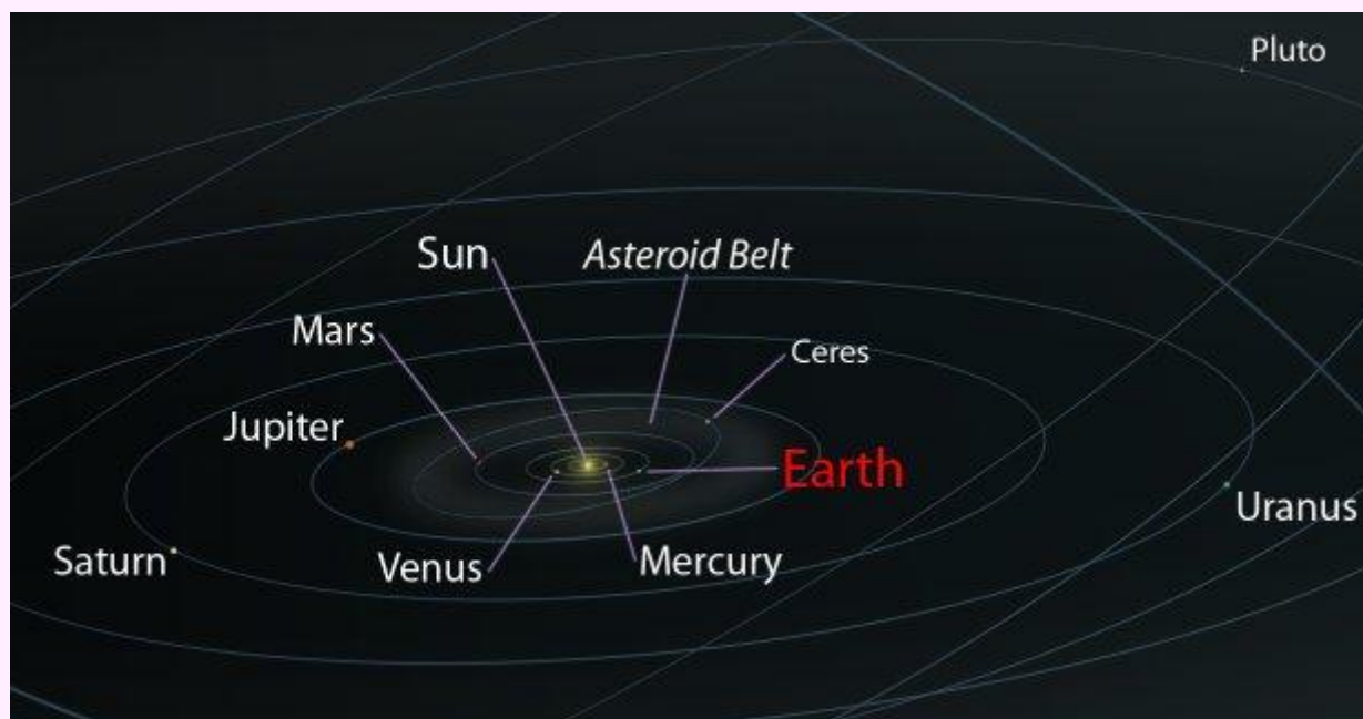
A cropped view of the solar system - See a larger view
